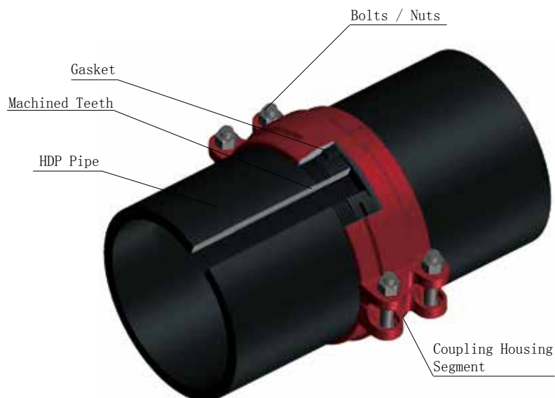
Model HDP Plain-End Coupling
