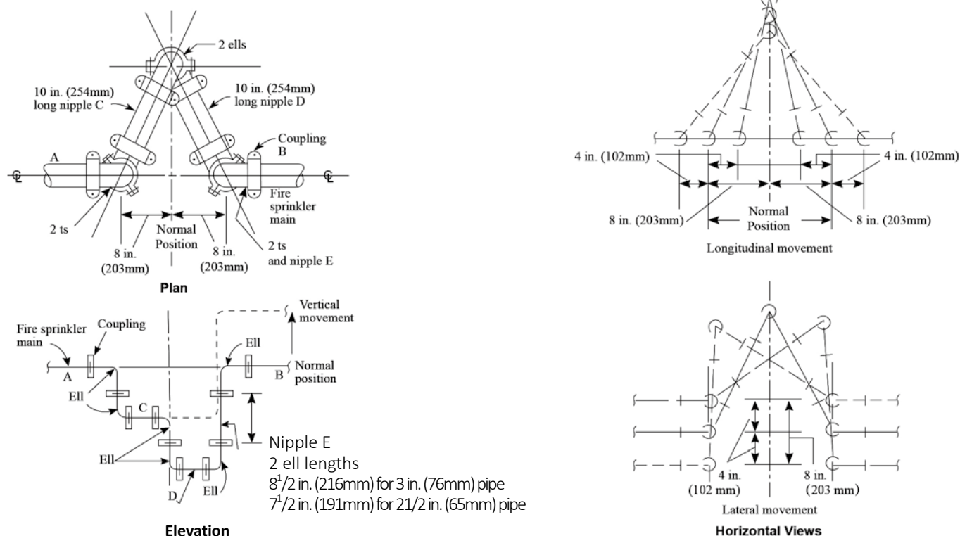
FIGURE A.9.3.3 (a) Seismic Separation Assembly. Shown are an 8 in. (203mm) Separation Crossed by Pipes up to 4 in. (102mm) in Nominal Diameter. For other separation distances and pipe sizes, lengths and distances should be modified proportionally.
